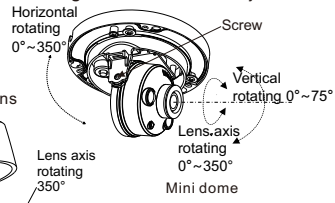
Figure 3-4 Three-axis adjustment
