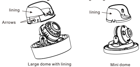
Figure 3-3 Removing lining
