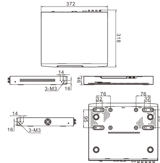
Figure 2-1 Dimensions (Unit:mm)
