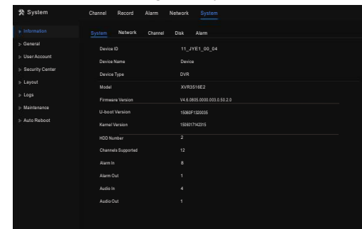
Figure 5-4 System
