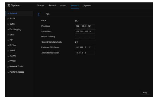
Figure 5-3 Network
