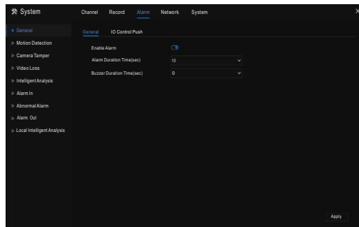
Figure 5-2 Alarm
