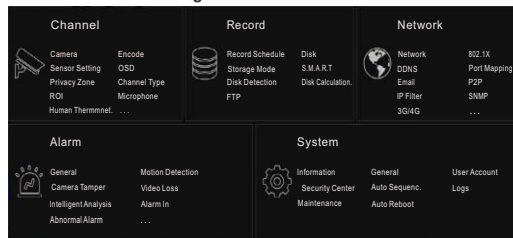
Figure 5-1 Main menu
