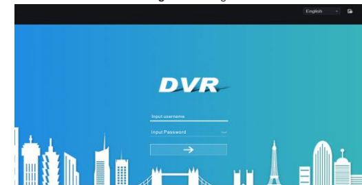
Figure 7-1 Login
