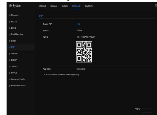
Figure 6-1 P2P
