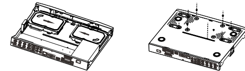
Figure 3-2 Installing hard disk Figure 3-3 Fixing hard disk
